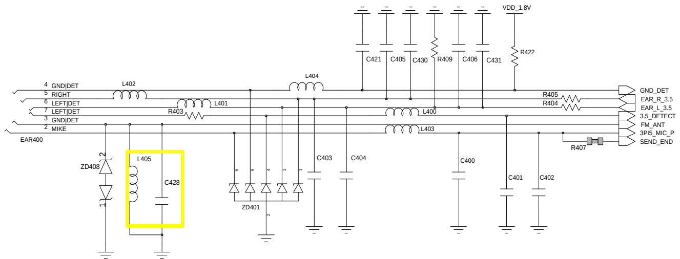
3.5 pi EAR JACK
